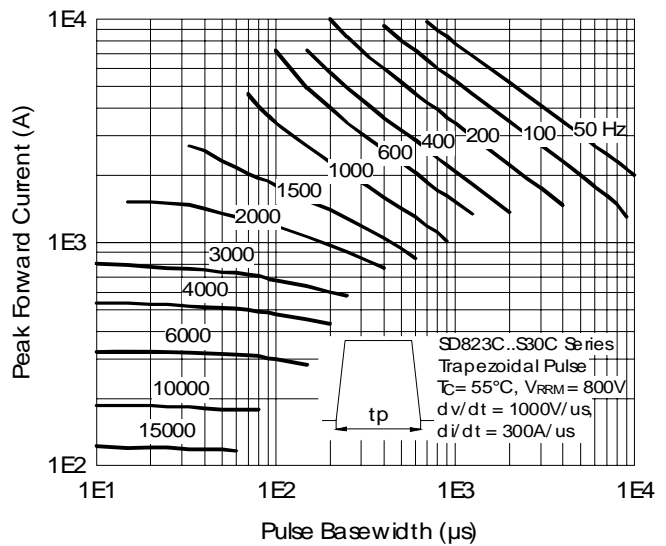
Fig. 37 - Frequency Characteristics
